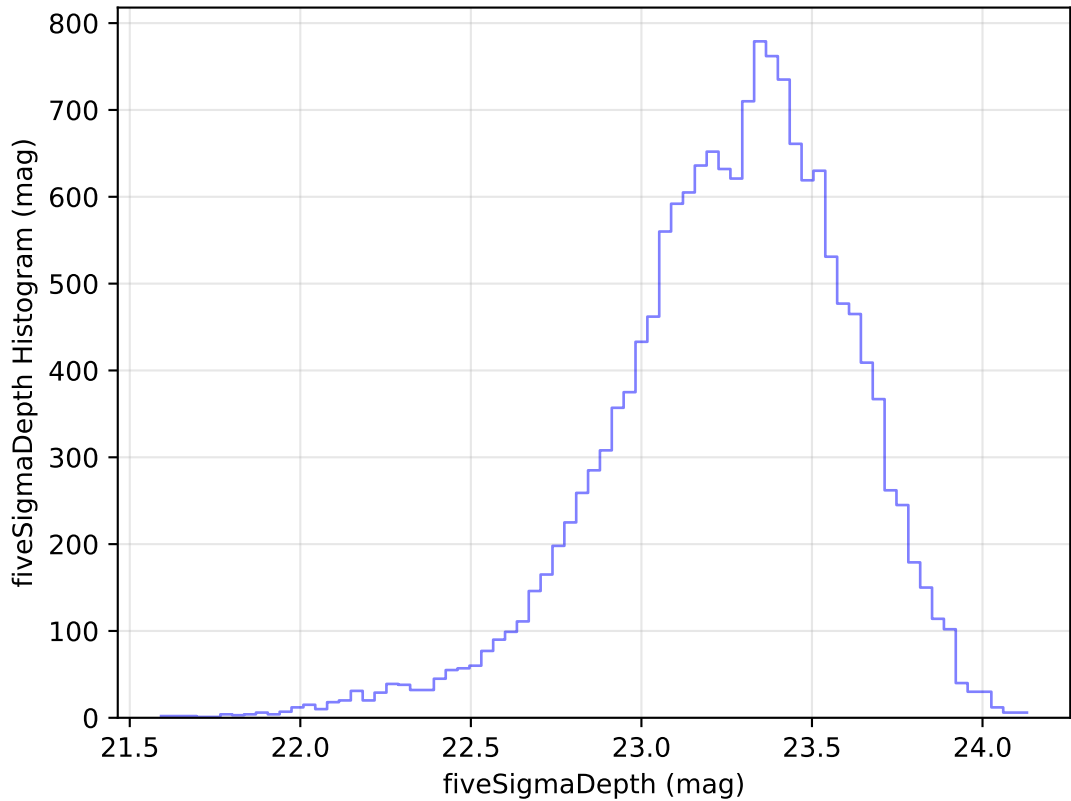
ddf_acor_sf20_lsf30_lsr50_v3.4_10yrs Yr 1 u band: fiveSigmaDepth Histogram
