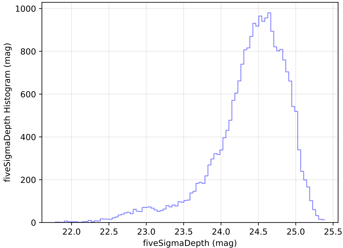
ddf_acor_sf20_lsf30_lsr50_v3.4_10yrs Yr 1 g band: fiveSigmaDepth Histogram
