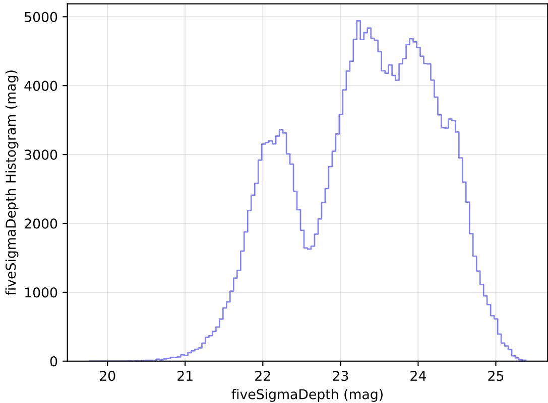
ddf_acor_sf20_Isf30_Isr50_v3.4_10yrs Yr 1 all bands: fiveSigmaDepth Histogram
