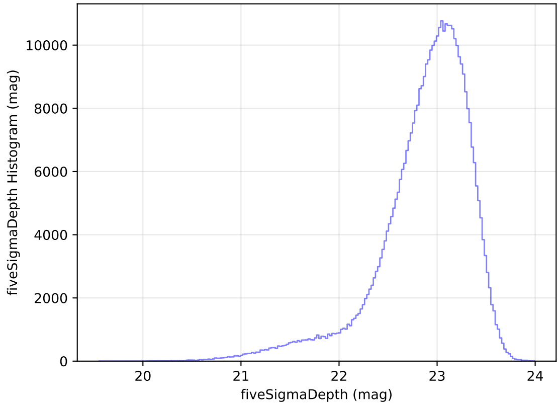
ddf_acor_sf20_lsf30_lsr50_v3.4_10yrs WFD z band: fiveSigmaDepth Histogram
