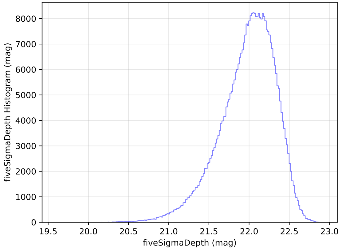
ddf_acor_sf20_lsf30_lsr50_v3.4_10yrs WFD y band: fiveSigmaDepth Histogram
