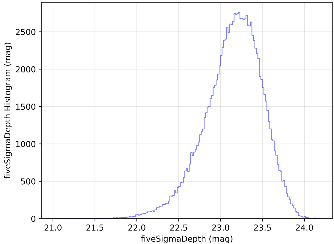
ddf_acor_sf20_lsf30_lsr50_v3.4_10yrs WFD u band: fiveSigmaDepth Histogram
