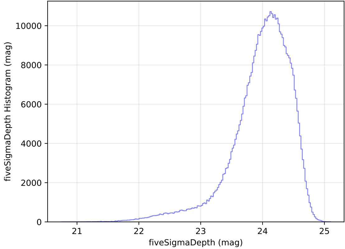
ddf_acor_sf20_lsf30_lsr50_v3.4_10yrs WFD r band: fiveSigmaDepth Histogram
