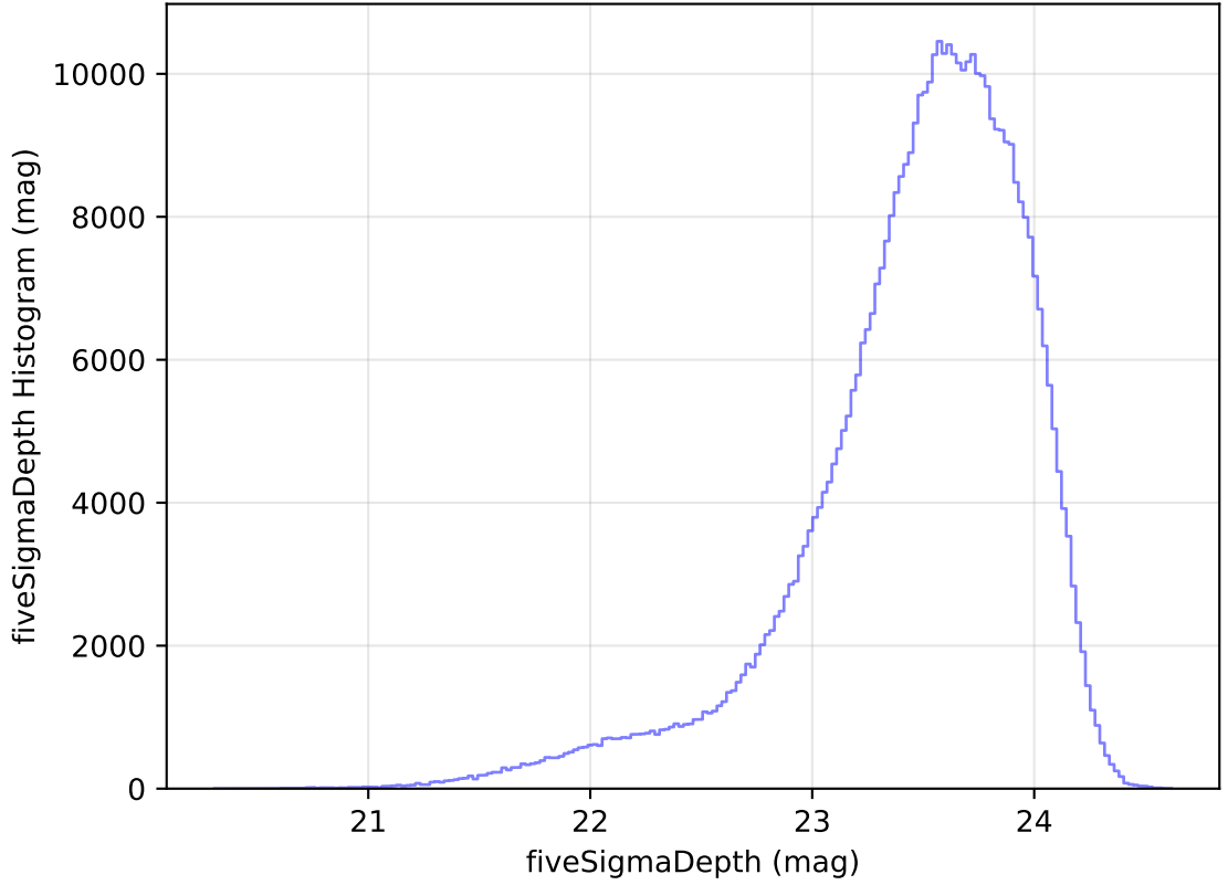
ddf_acor_sf20_lsf30_lsr50_v3.4_10yrs WFD i band: fiveSigmaDepth Histogram
