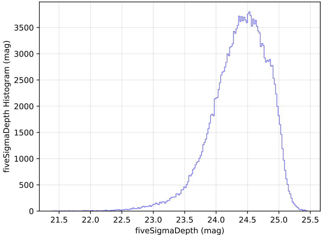
ddf_acor_sf20_lsf30_lsr50_v3.4_10yrs WFD g band: fiveSigmaDepth Histogram
