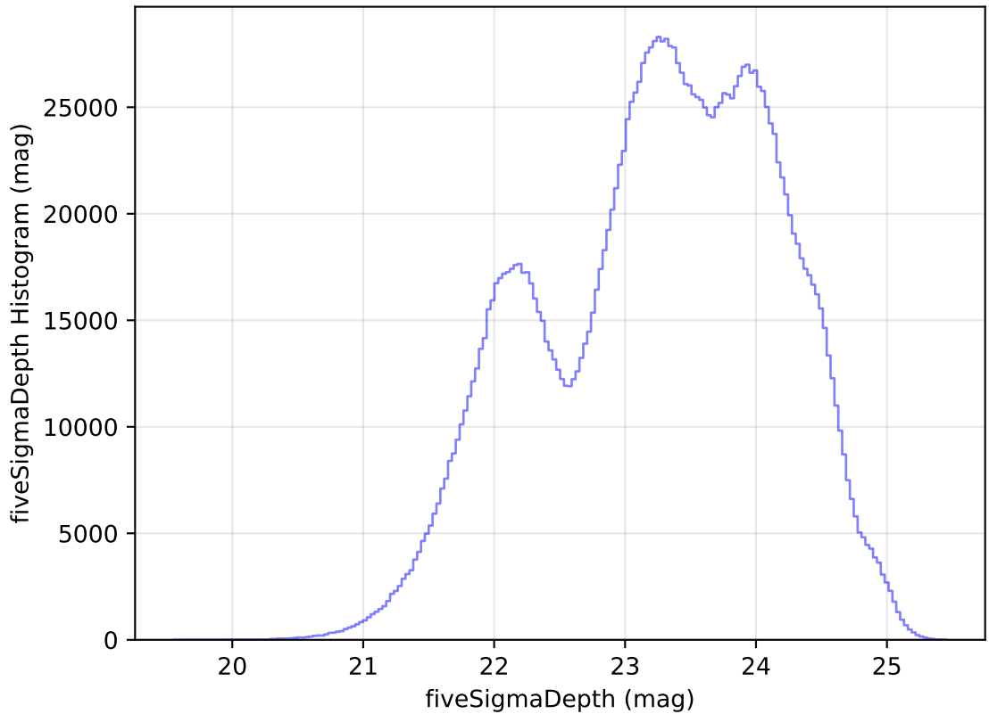
ddf_acor_sf20_lsf30_lsr50_v3.4_10yrs WFD all bands: fiveSigmaDepth Histogram
