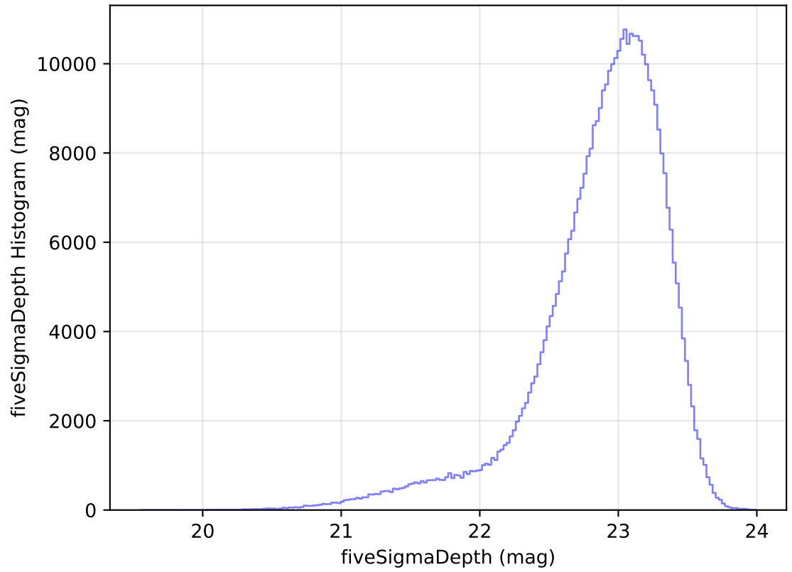
ddf_acor_sf20_lsf30_lsr50_v3.4_10yrs All sky z band: fiveSigmaDepth Histogram
