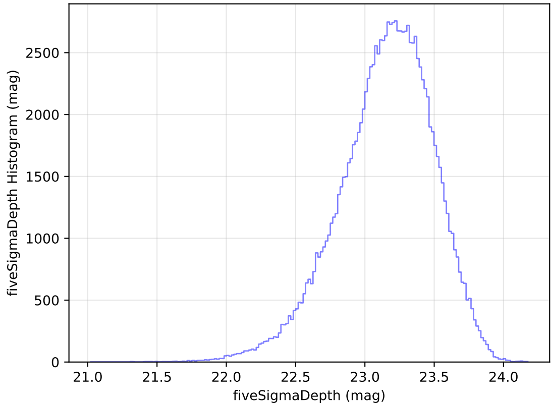
ddf_acor_sf20_lsf30_lsr50_v3.4_10yrs All sky u band: fiveSigmaDepth Histogram
