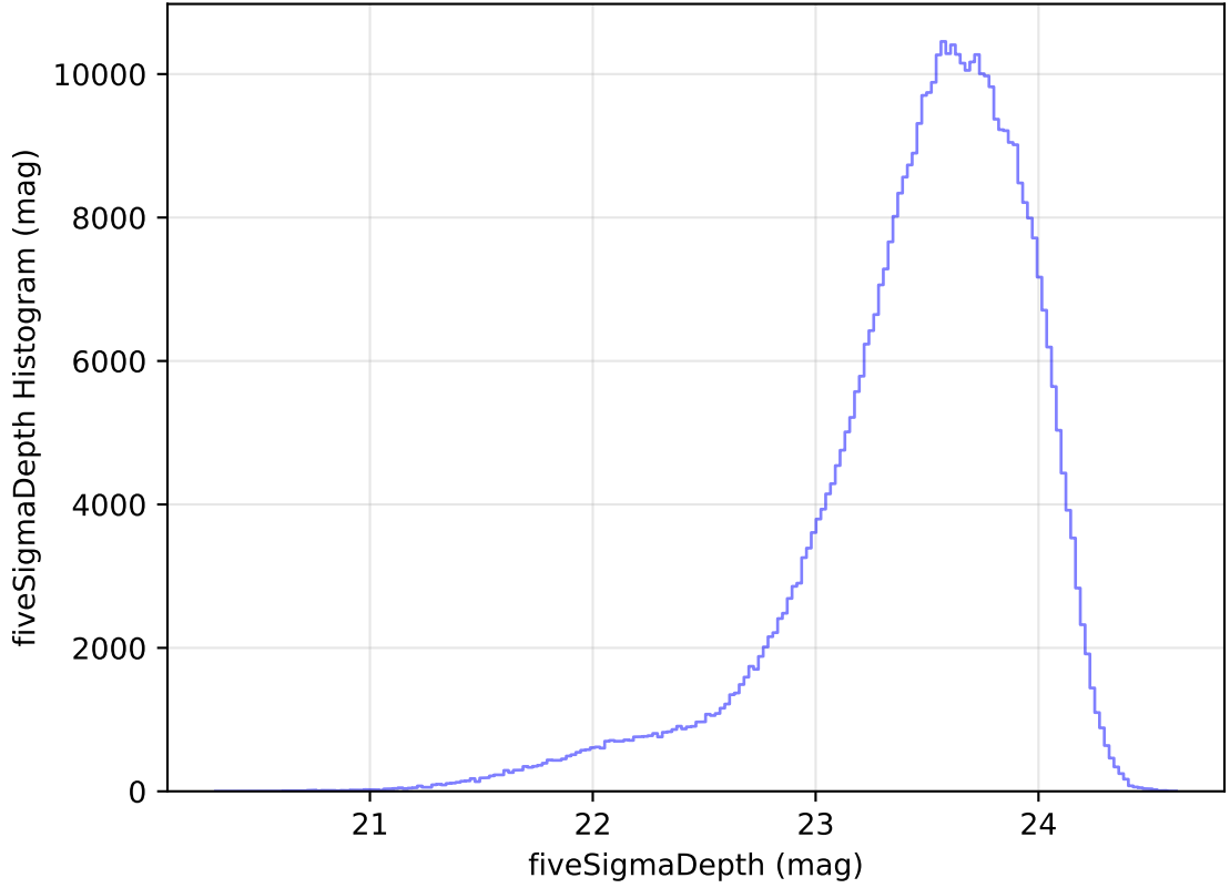
ddf_acor_sf20_lsf30_lsr50_v3.4_10yrs All sky i band: fiveSigmaDepth Histogram
