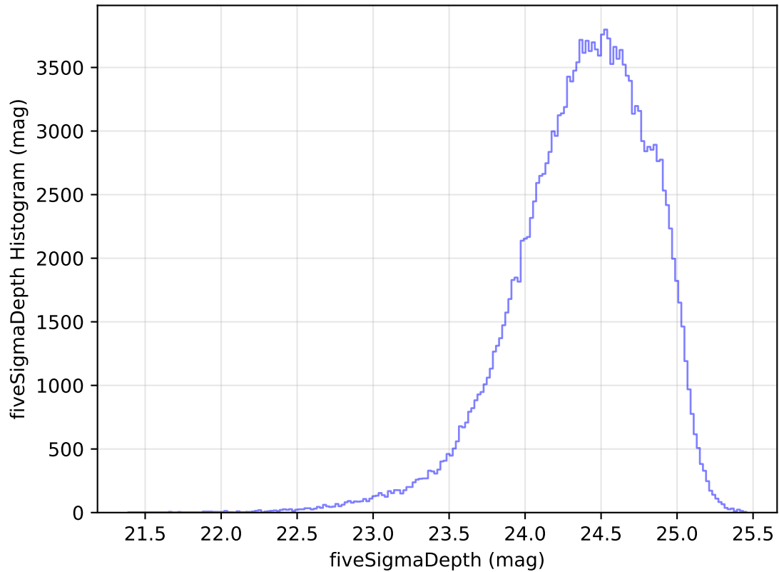
ddf_acor_sf20_lsf30_lsr50_v3.4_10yrs All sky g band: fiveSigmaDepth Histogram
