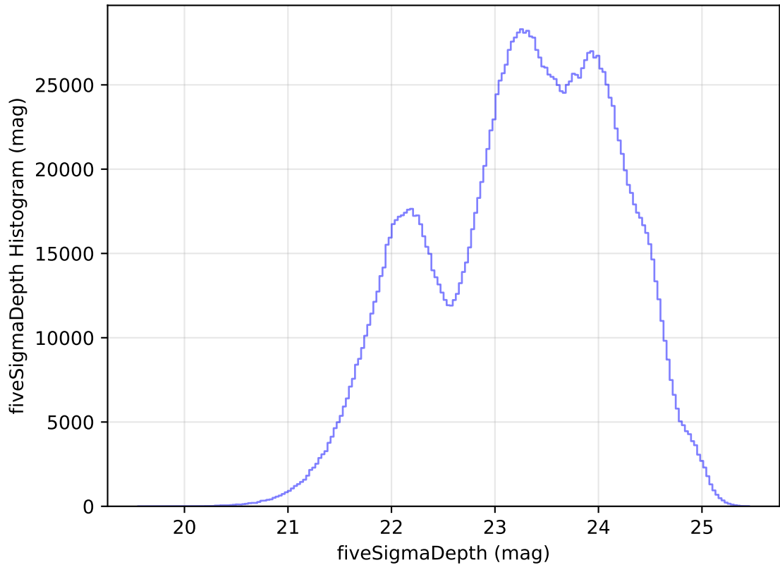
ddf_acor_sf20_lsf30_lsr50_v3.4_10yrs All sky all bands: fiveSigmaDepth Histogram
