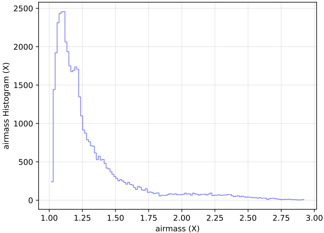
ddf_acor_sf20_lsf30_lsr50_v3.4_10yrs Yr 1 z band: airmass Histogram
