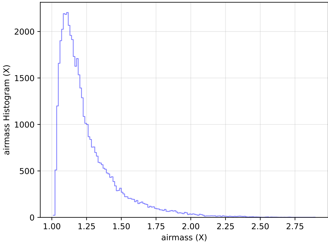
ddf_acor_sf20_lsf30_lsr50_v3.4_10yrs Yr 1 y band: airmass Histogram
