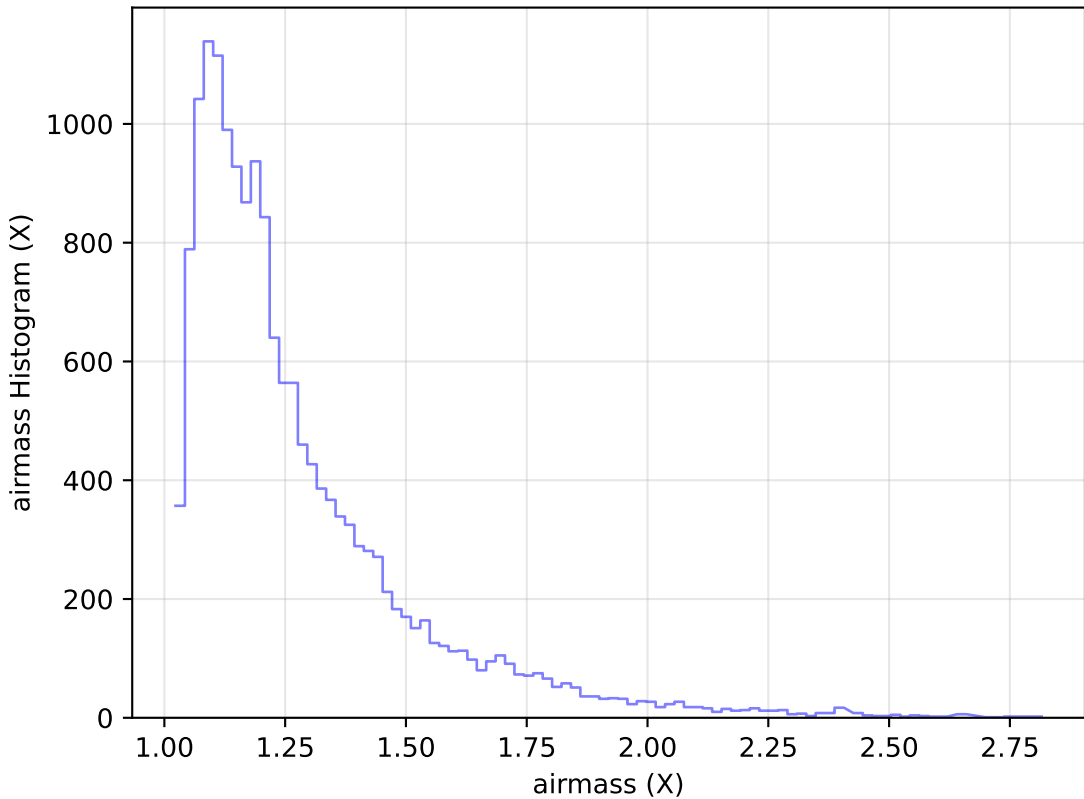
ddf_acor_sf20_lsf30_lsr50_v3.4_10yrs Yr 1 u band: airmass Histogram
