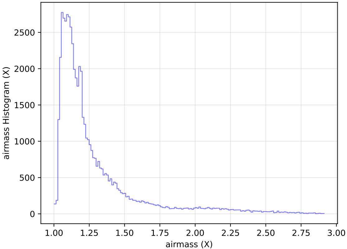
ddf_acor_sf20_lsf30_lsr50_v3.4_10yrs Yr 1 i band: airmass Histogram
