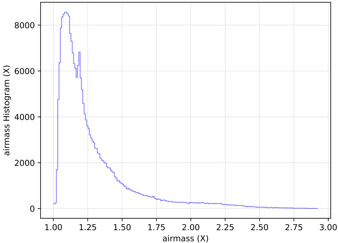
ddf_acor_sf20_lsf30_lsr50_v3.4_10yrs Yr 1 all bands: airmass Histogram
