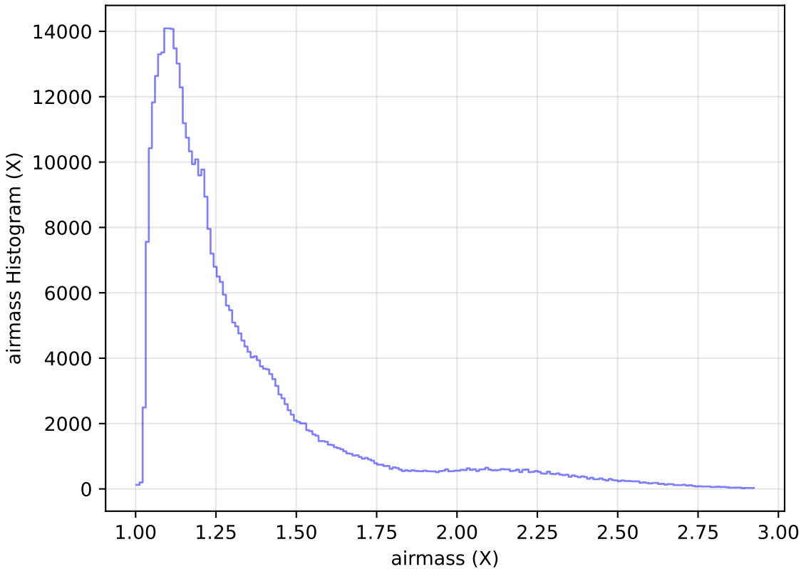
ddf_acor_sf20_lsf30_lsr50_v3.4_10yrs WFD z band: airmass Histogram
