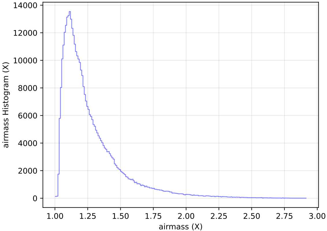
ddf_acor_sf20_lsf30_lsr50_v3.4_10yrs WFD y band: airmass Histogram
