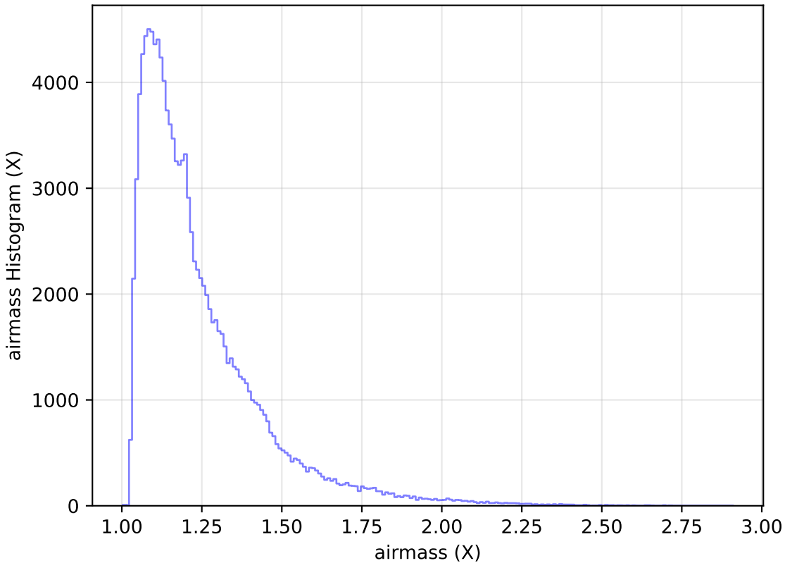
ddf_acor_sf20_lsf30_lsr50_v3.4_10yrs WFD u band: airmass Histogram
