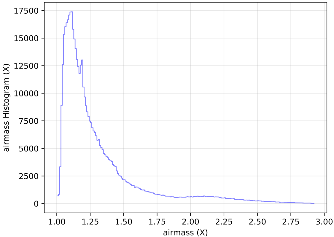
ddf_acor_sf20_lsf30_lsr50_v3.4_10yrs WFD i band: airmass Histogram
