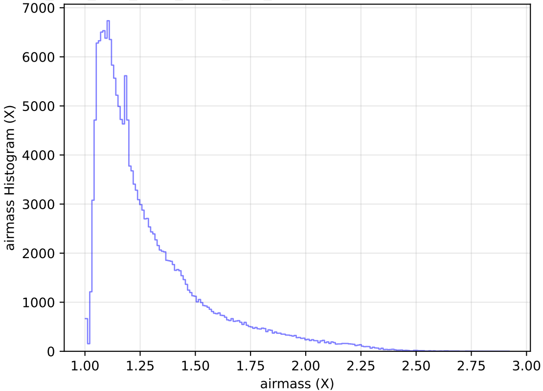
ddf_acor_sf20_lsf30_lsr50_v3.4_10yrs WFD g band: airmass Histogram
