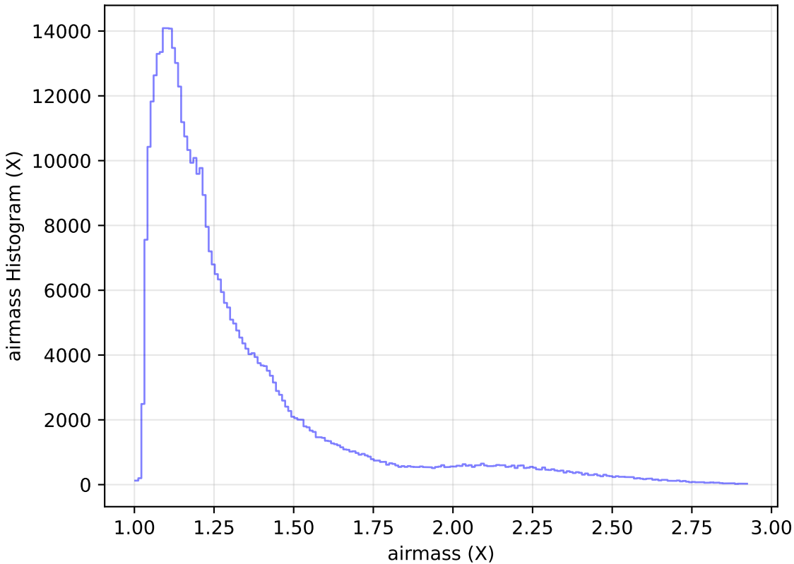
ddf_acor_sf20_lsf30_lsr50_v3.4_10yrs All sky z band: airmass Histogram
