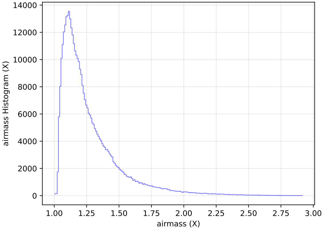
ddf_acor_sf20_lsf30_lsr50_v3.4_10yrs All sky y band: airmass Histogram
