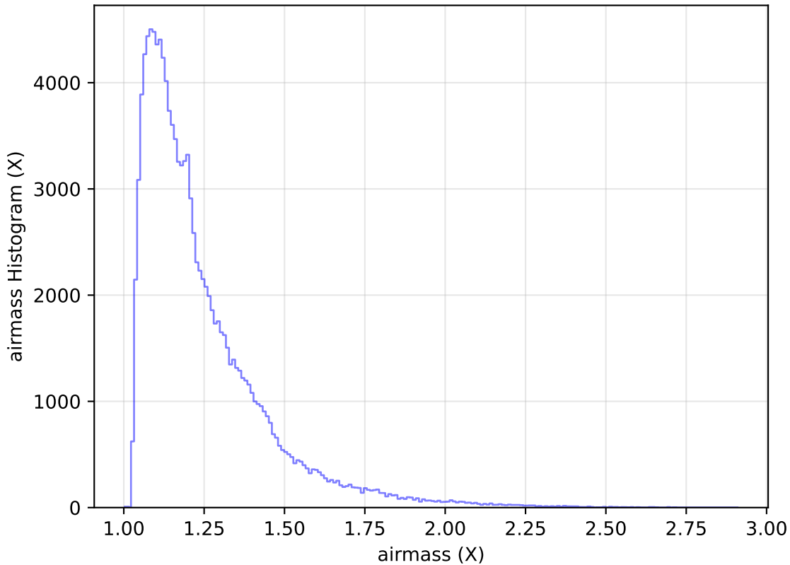
ddf_acor_sf20_lsf30_lsr50_v3.4_10yrs All sky u band: airmass Histogram
