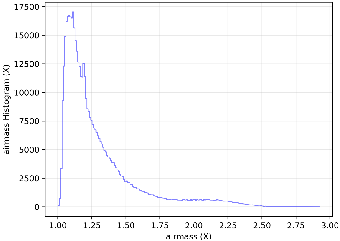
ddf_acor_sf20_lsf30_lsr50_v3.4_10yrs All sky r band: airmass Histogram
