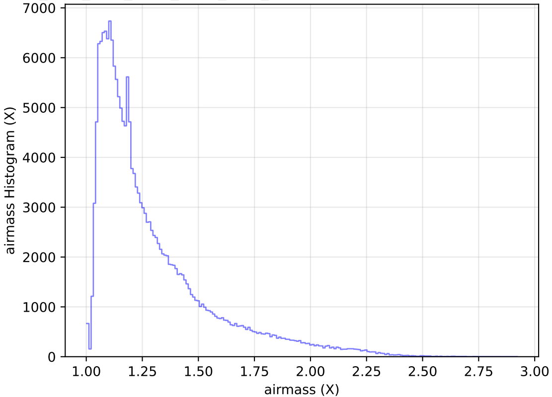
ddf_acor_sf20_lsf30_lsr50_v3.4_10yrs All sky g band: airmass Histogram
