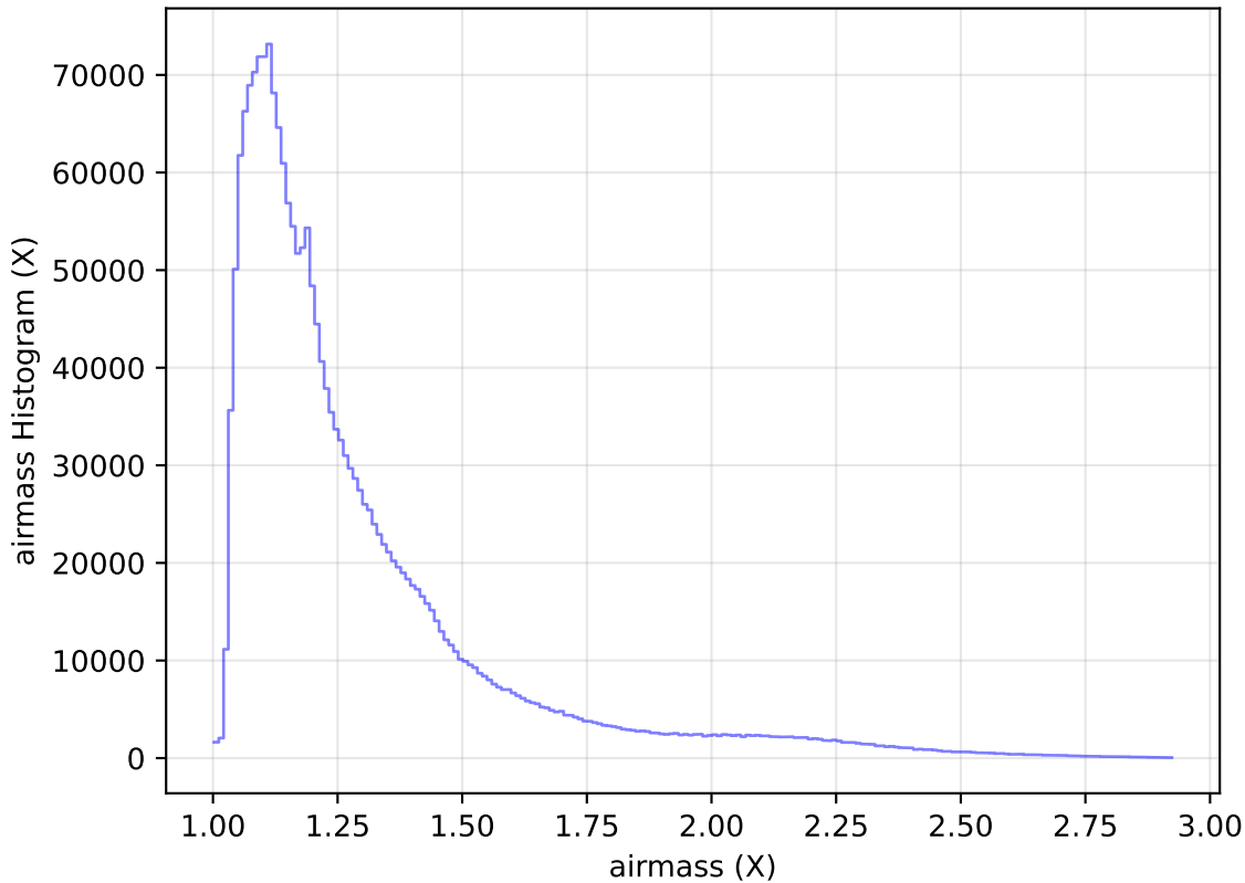
ddf_acor_sf20_lsf30_lsr50_v3.4_10yrs All sky all bands: airmass Histogram
