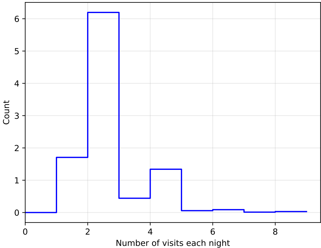
ddf_acor_sf20_lsf30_lsr50_v3.4_10yrs All sky: NVisitsPerNight 1e6
