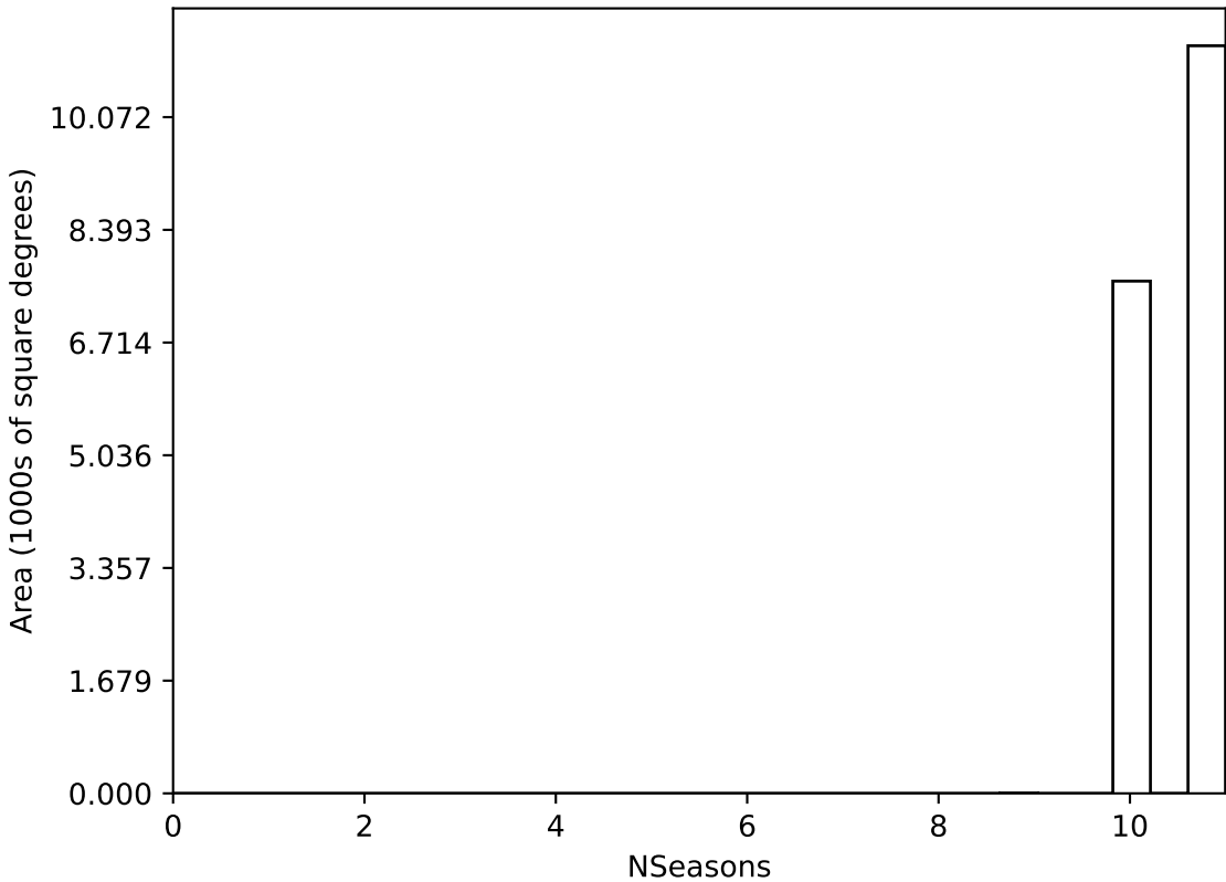
ddf_acor_sf20_lsf30_lsr50_v3.4_10yrs WFD all bands: NSeasons
