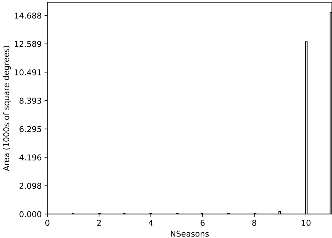
ddf_acor_sf20_lsf30_lsr50_v3.4_10yrs All sky all bands: NSeasons
