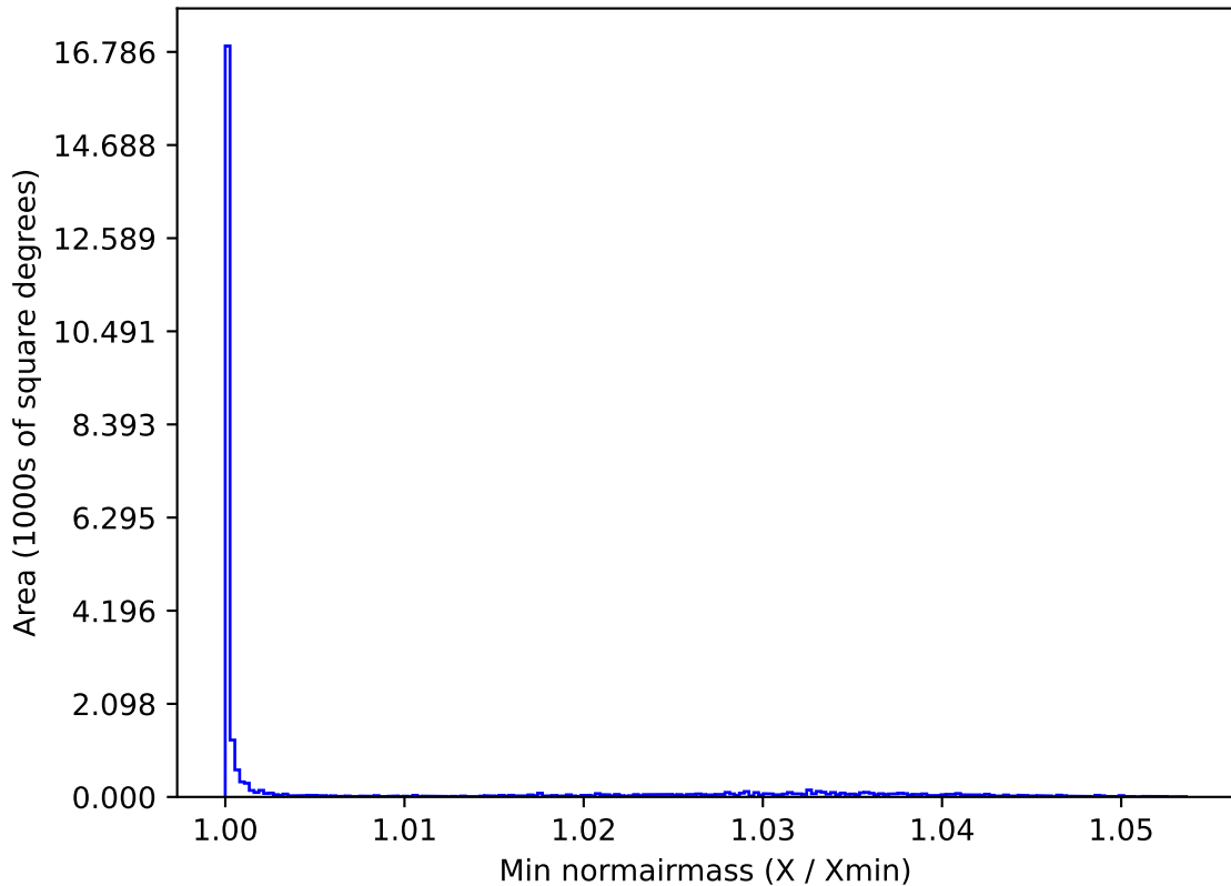
ddf_acor_sf20_lsf30_lsr50_v3.4_10yrs All sky g band: Min normairmass
