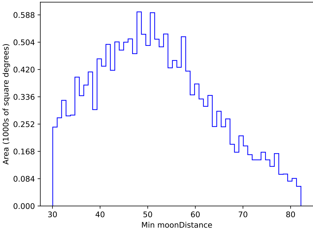
ddf_acor_sf20_lsf30_lsr50_v3.4_10yrs WFD u band: Min moonDistance
