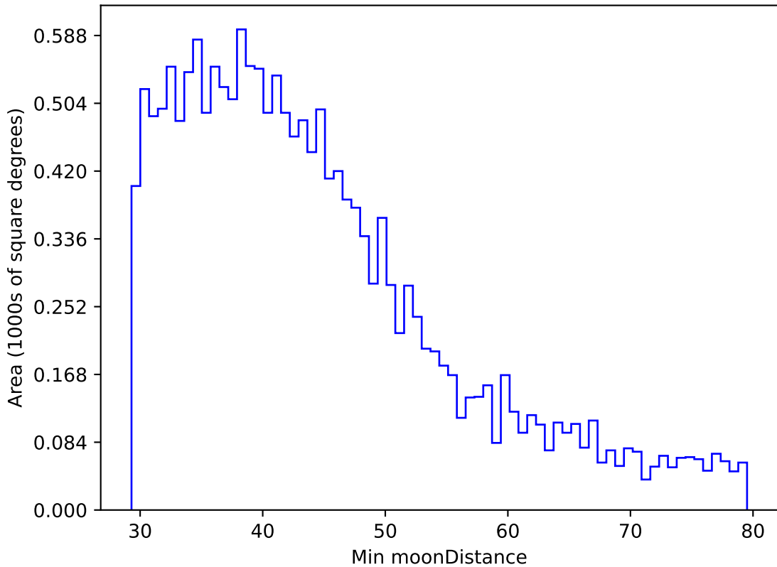
ddf_acor_sf20_lsf30_lsr50_v3.4_10yrs WFD g band: Min moonDistance
