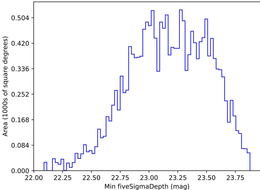
ddf_acor_sf20_lsf30_lsr50_v3.4_10yrs WFD g band: Min fiveSigmaDepth
