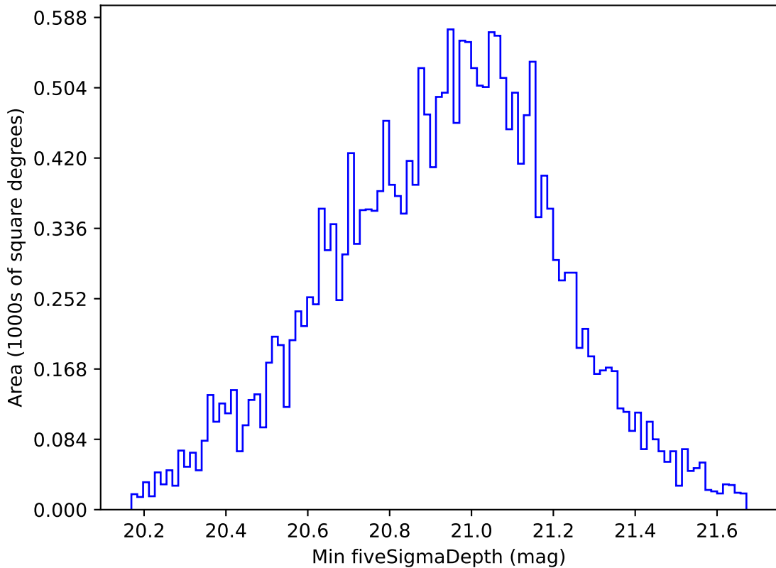
ddf_acor_sf20_lsf30_lsr50_v3.4_10yrs All sky y band: Min fiveSigmaDepth
