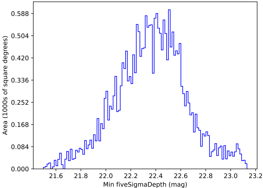
ddf_acor_sf20_lsf30_lsr50_v3.4_10yrs All sky u band: Min fiveSigmaDepth
