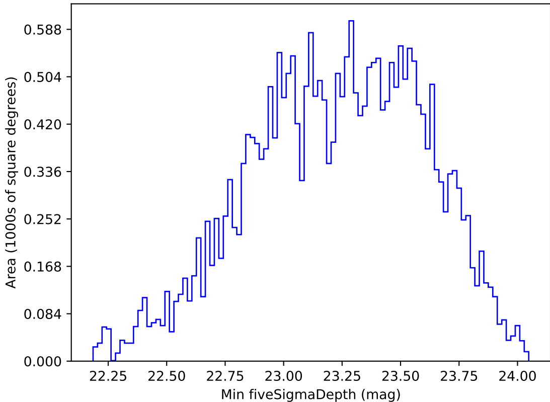
ddf_acor_sf20_lsf30_lsr50_v3.4_10yrs All sky g band: Min fiveSigmaDepth
