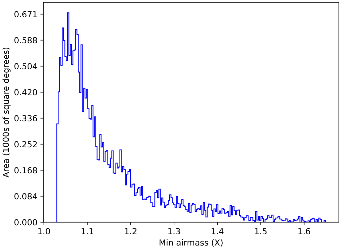
ddf_acor_sf20_lsf30_lsr50_v3.4_10yrs Yr 1 u band: Min airmass
