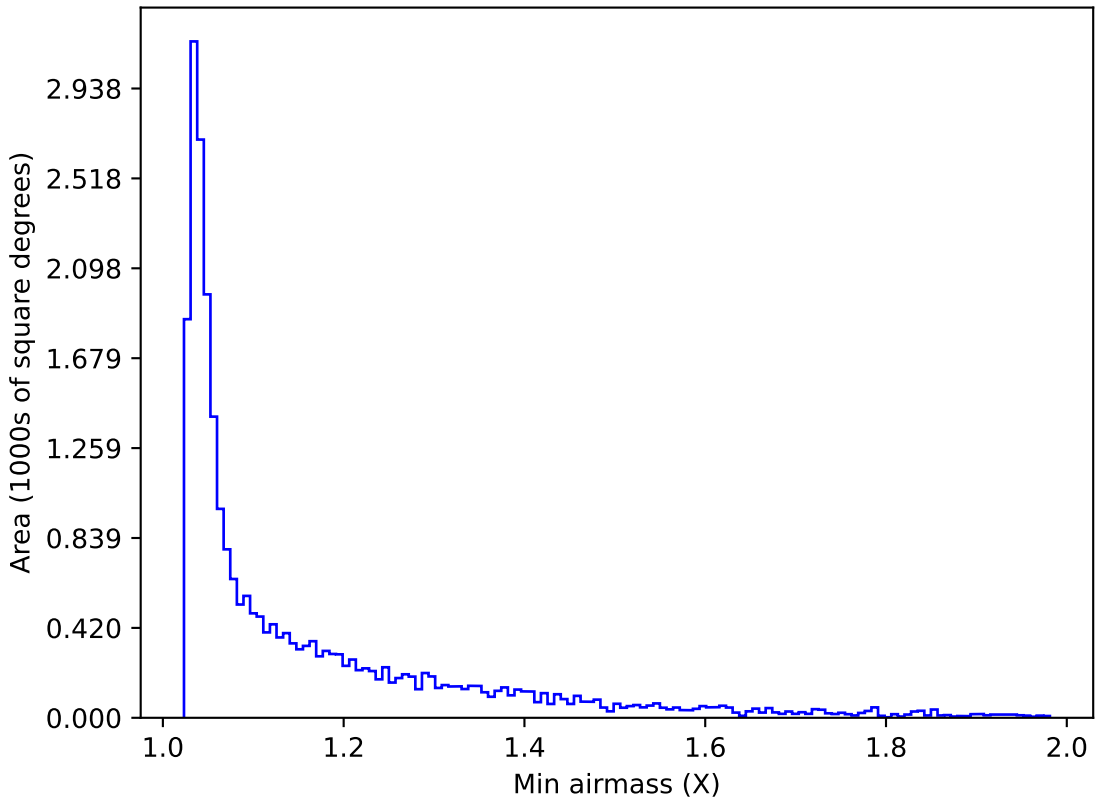
ddf_acor_sf20_lsf30_lsr50_v3.4_10yrs Yr 1 r band: Min airmass
