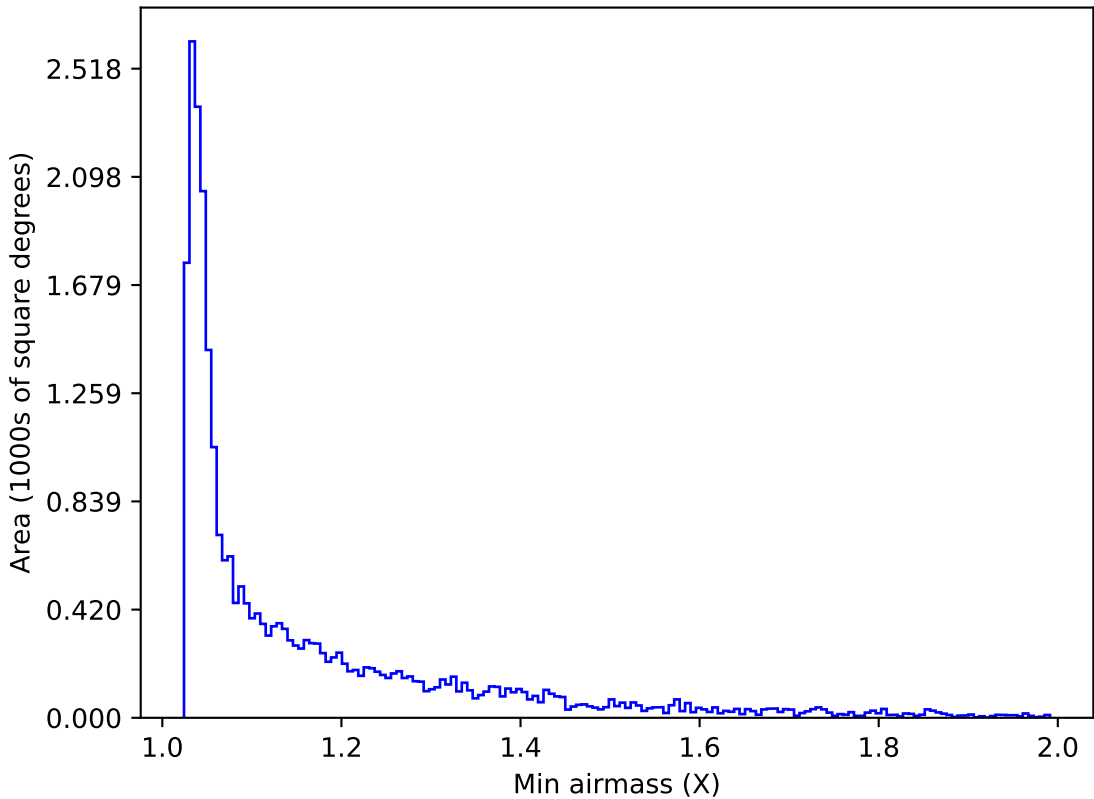
ddf_acor_sf20_lsf30_lsr50_v3.4_10yrs Yr 1 i band: Min airmass
