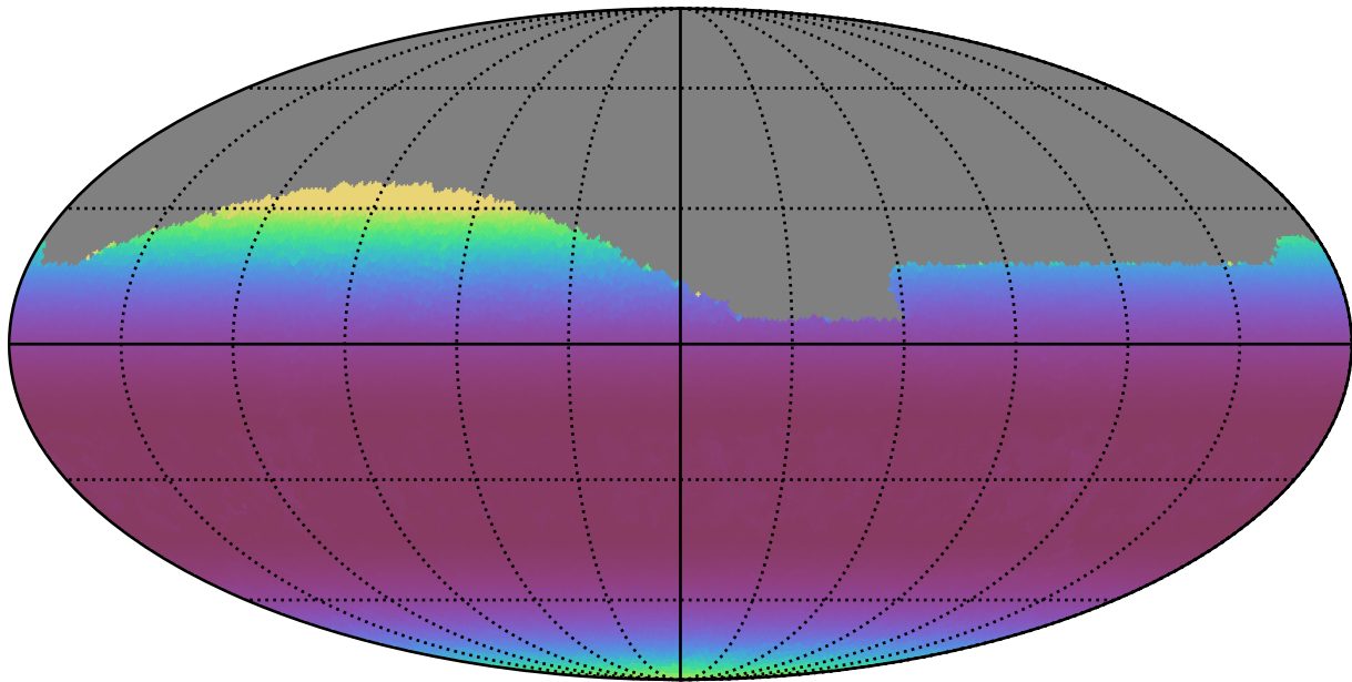
ddf_acor_sf20_lsf30_lsr50_v3.4_10yrs Yr 1 all bands: Min airmass
