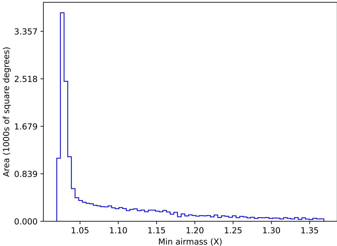
ddf_acor_sf20_lsf30_lsr50_v3.4_10yrs WFD z band: Min airmass
