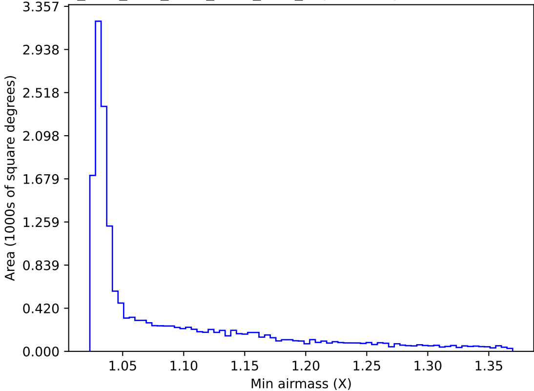
ddf_acor_sf20_lsf30_lsr50_v3.4_10yrs WFD y band: Min airmass
