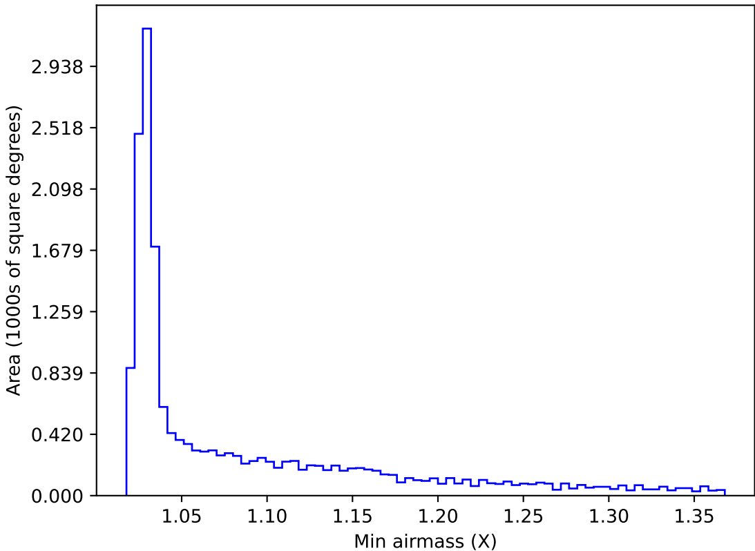
ddf_acor_sf20_lsf30_lsr50_v3.4_10yrs WFD i band: Min airmass
