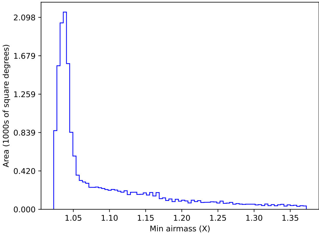
ddf_acor_sf20_lsf30_lsr50_v3.4_10yrs WFD g band: Min airmass
