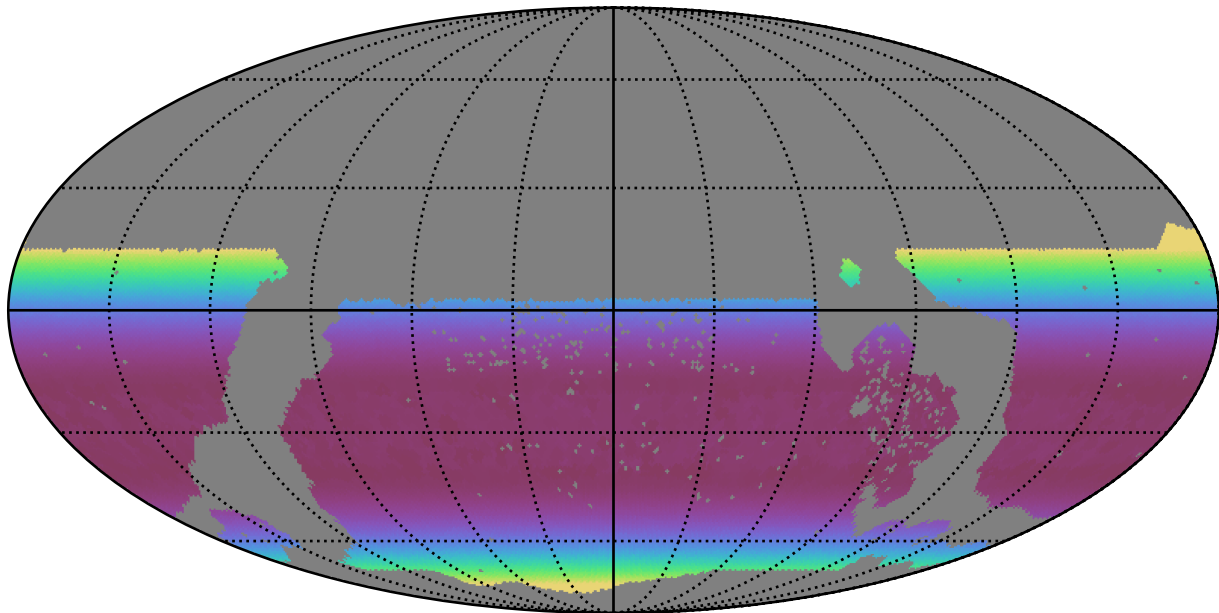
ddf_acor_sf20_lsf30_lsr50_v3.4_10yrs WFD all bands: Min airmass
